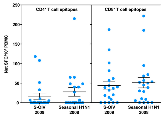
Fig. 4. Comparable pre-existing CD4 + and CD8 + T-cell immunity to S-OIV and 2008 seasonal influenza. PBMC from normal individuals ( n = 20 ) were stimulated with pools of either CD4 + or CD8 + T-cell epitopes that were conserved in S-OIV or seasonal influenza 2008 sequences. Responses were measured through ex vivo IFN- \gamma ELISPOT assays. Error bars represent SEM.
