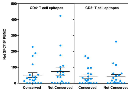
Fig. 2. Detection of pre-existing CD4 + and CD8 + T-cell immune responses to S-OIV. PBMC from normal individuals ( n = 20 ) were stimulated with pools of either CD4 + or CD8 + T-cell epitopes from recent seasonal H1N1 influenza strains that were either absolutely conserved or not conserved in S-OIV sequences. Responses were measured through ex vivo IFN-γ ELISPOT assays. Error bars represent SEM.
