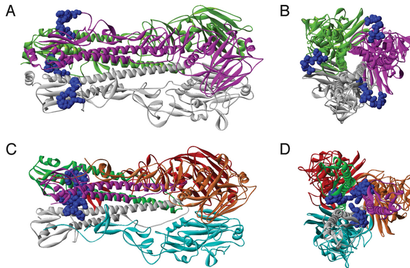
Fig. 1. Location of the conserved epitope in the S-OIV HA protein structure. (A and B) Quaternary structure of the HA precursor (Protein Data Bank ID: 1HA0): frontal (A) and orthogonal (B) views. Monomer chains are in white, magenta, and green. Epitopes in each monomer are identical and shown in blue. (C and D) Quaternary structure of the cleaved HA modeled for the representative swine influenza HA sequence (ACP41934.1): frontal (C) and orthogonal (D) views. HA2 chains are in white, magenta, and green; corresponding HA1 chains are in cyan, orange, and red. Epitope is located at the N-terminal of HA2 chain and is identical in each chain.
