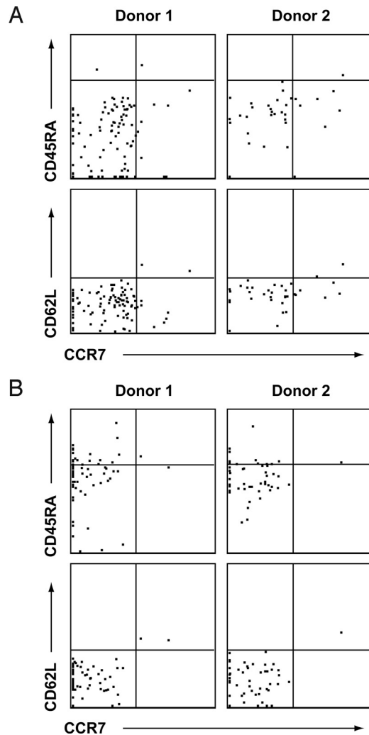
Fig. 3. S-OIV-specific CD4 + and CD8 + T cells appear to have an effector memory phenotype. PBMC from two representative normal donors were stimulated with either pools of (A) CD4 + or (B) CD8 + T-cell epitopes conserved in S-OIV sequences. The cells were gated for IFN- \gamma production and presence of the surface markers CD4 and CD8, respectively. Signal intensities of the gated cells for memory phenotypic markers CD45RA, CD62L, and CCR7 are shown.
